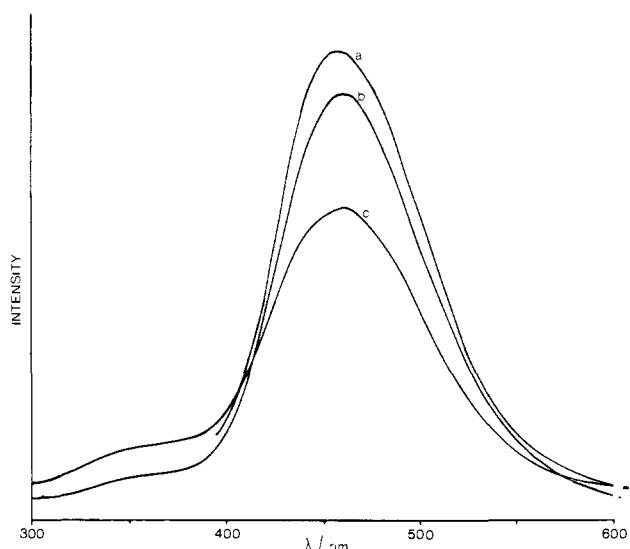
Figure 9. Fluorescence of aqueous salicylanilide ( 7 \times 10^{-5} M) at pH 0.3. Excitation wavelengths (nm): (a) 330; (b) 300; (c) 265.
