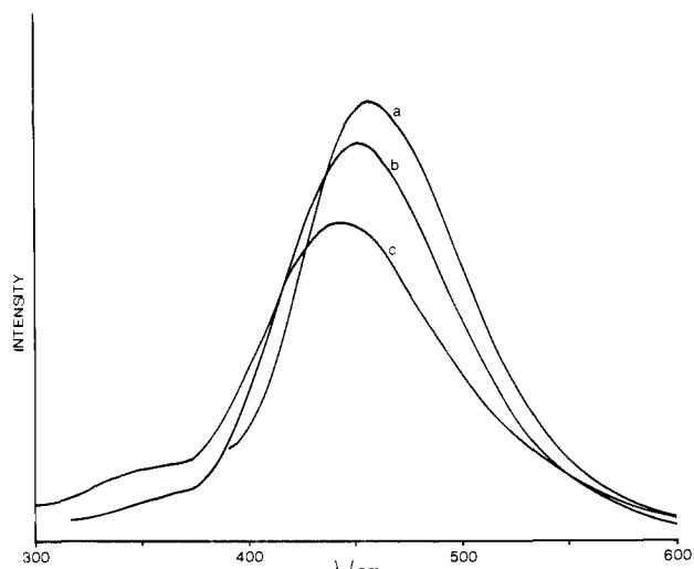
Figure 8. Fluorescence of aqueous salicylanilide ( 7 \times 10^{-5} M) at pH 3. Excitation wavelengths (nm): (a) 330; (b) 300; (c) 265.
