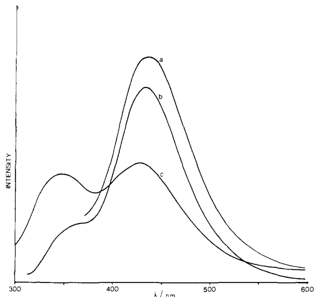
Figure 6. Fluorescence of salicylamide in D_2O ( 1.7 \times 10^{-4} M). Excitation wavelengths (nm): (a) 330; (b) 300; (c) 265.
