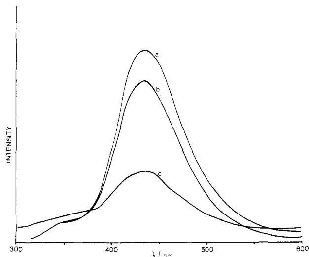
Figure 3. Fluorescence of aqueous salicylamide ( 1 \times 10^{-4} M) at pH 0.3. Excitation wavelengths (nm): (a) 330; (b) 300; (c) 265.
