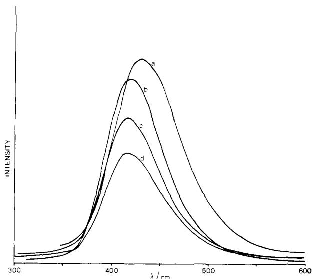
Figure 2. Fluorescence of aqueous salicylamide ( 1 \times 10^{-4} M) at pH 3. Excitation wavelengths (nm): (a) 330; (b) 300; (c) 265; (d) 230. (Raman scatter peaks have been removed.) Intensities have been adjusted for the sake of clarity.
