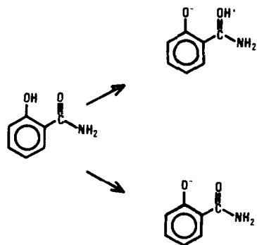
Figure 1. Excited-state reaction scheme for aqueous salicylamide.
