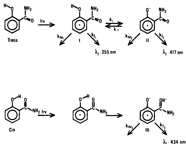
Figure 5. Proposed photochemical scheme for aqueous salicylamide.
