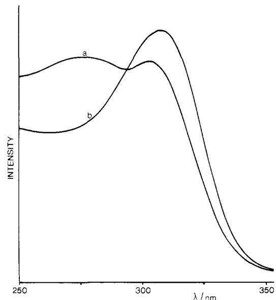
Figure 10. Fluorescence excitation spectra for aqueous salicylanilide at pH 3. Emission wavelengths (nm): (a) 425; (b) 490.
