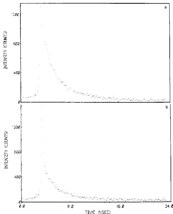
Figure 4. Fluorescence decay curves for aqueous salicylamide ( 1 \times 10^{-3} M): (a) \lambda_{em} = 400\text{--}430 nm; (b) \lambda_{em} \geq 495 nm.
