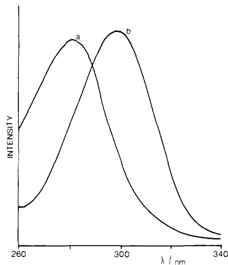
Figure 7. Fluorescence excitation spectra for salicylamide in D_2O . Emission wavelengths (nm): (a) 350; (b) 430.
